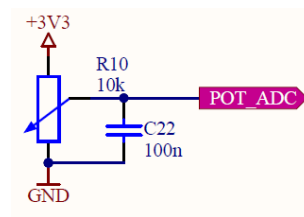
Picture 19: ADC Pot circuit
