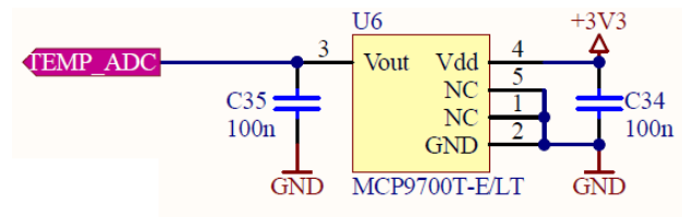
Picture 14: Temperature sensor circuit
