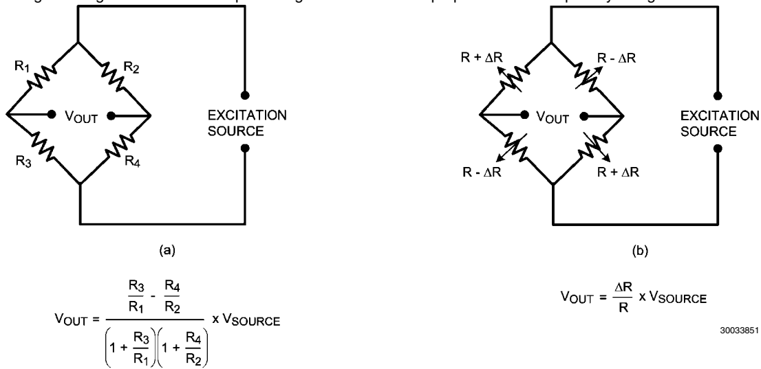
FIGURE 4. Bridge Sensor
