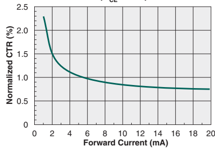
Darlington Transistor Normalized CTR vs. Forward Current ( V_{CE}=0.8V )
