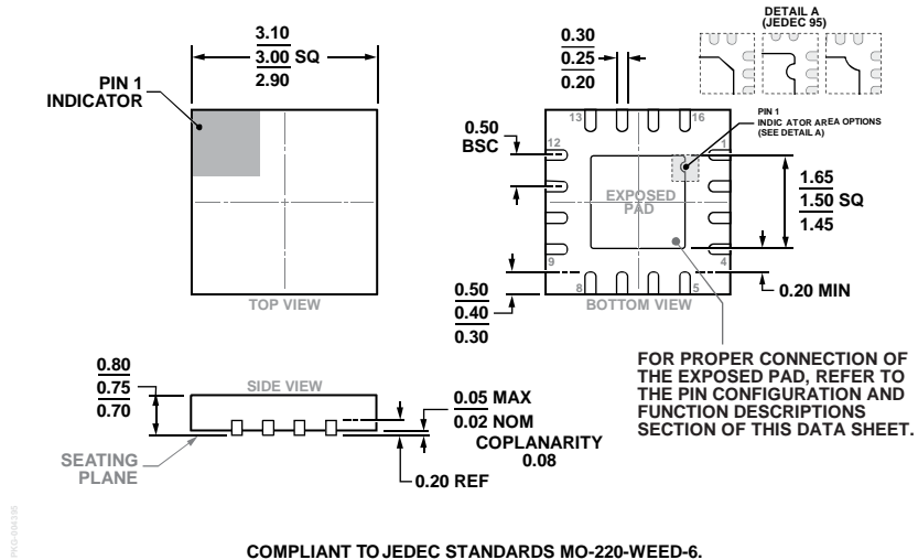
Figure 51. 16-Lead Lead Frame Chip Scale Package [LFCSPP] 3 mm × 3 mm Body and 0.75 mm Package Height (CP-16-27) Dimensions in millimeters
