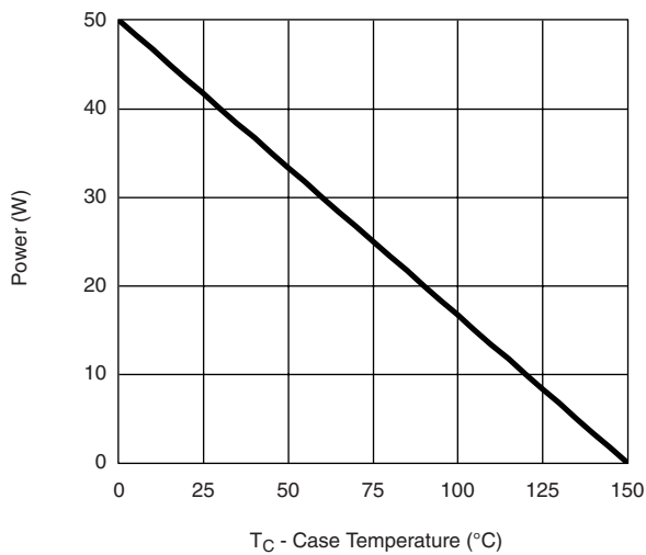
Power, Junction-to-Case
