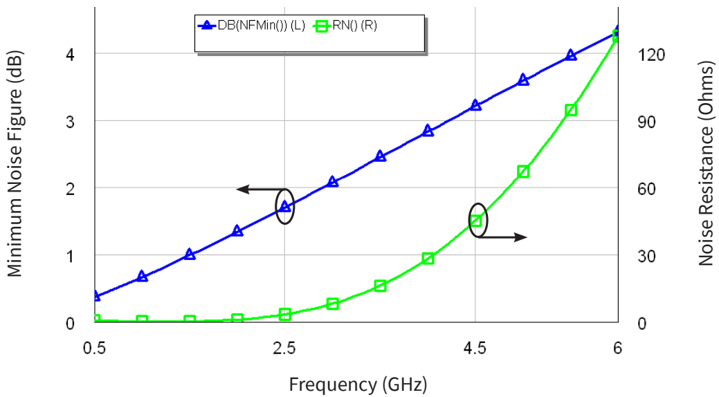
Simulated Minimum Noise Figure and Noise Resistance vs Frequency of the CGH40120F V_{DD} = 28\text{ V}, I_{DQ} = 1\text{ A}
