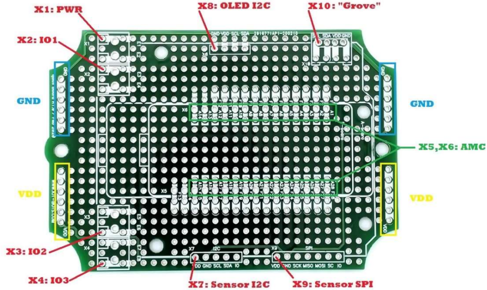
Pic.11. Connectors placement proposal: Arduino MKR Compatible board based
