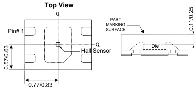
Sensor Location
