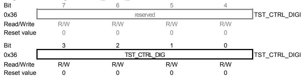
Figure A-1. Register TST_CTRL_DIGI.
