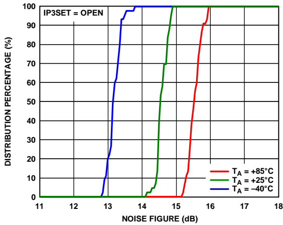
Figure 28. Noise Figure
