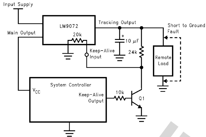
FIGURE 6. Safety Latch-OFF
