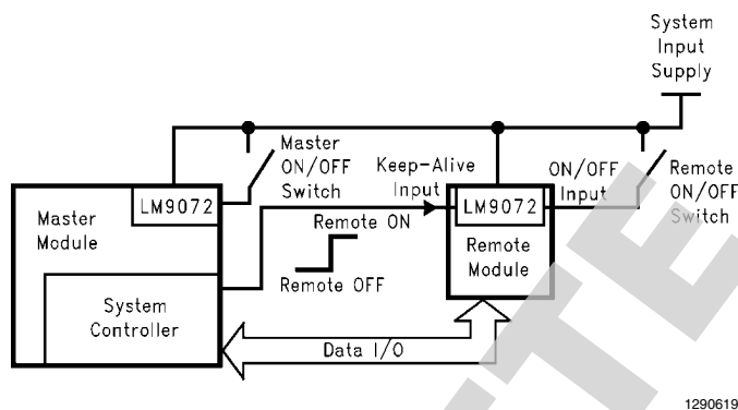
FIGURE 3. Remote ON/OFF Control
