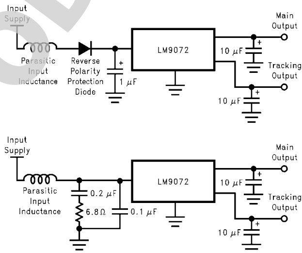
FIGURE 7. Input Bypassing
