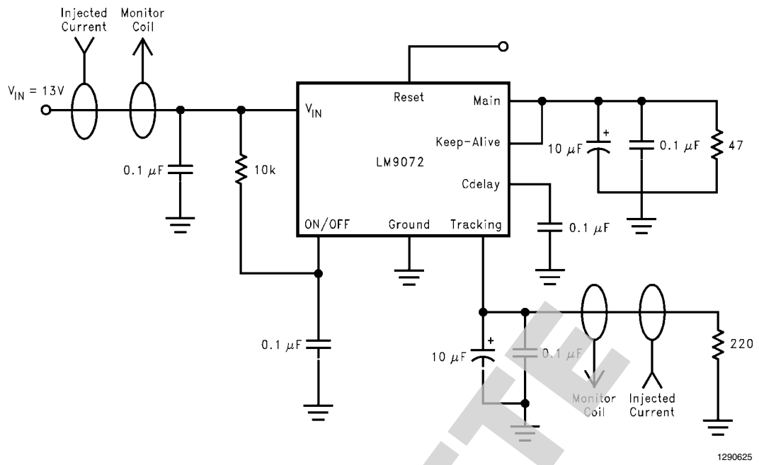
FIGURE 9. Bulk Current Injection Test Configuration
