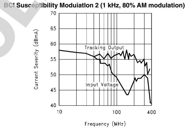
FIGURE 10. Examples of BCI Test Results
