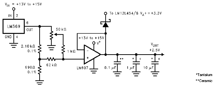
FIGURE 12. Low Drift Extremely Stable Reference Circuit
