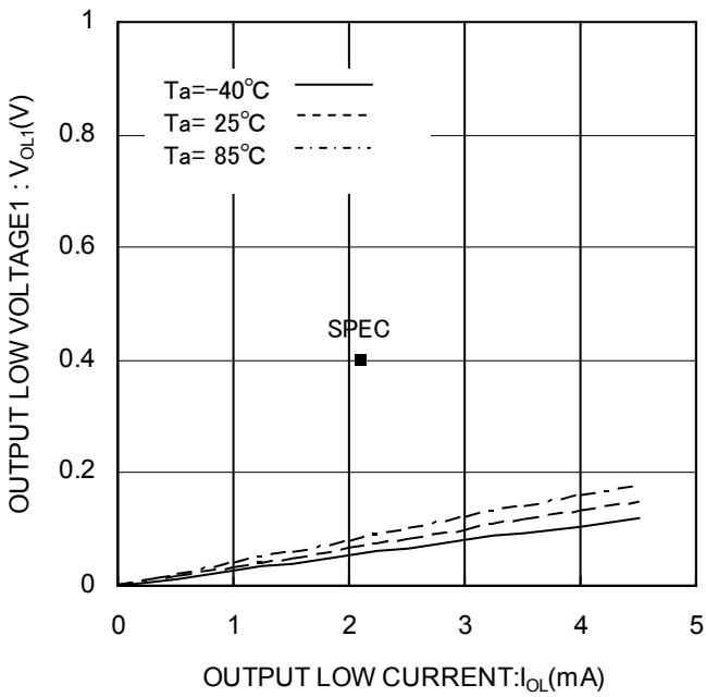
Figure 6. Output low voltage1 V_{O1} ( V_{CC}=2.7\text{V} )
