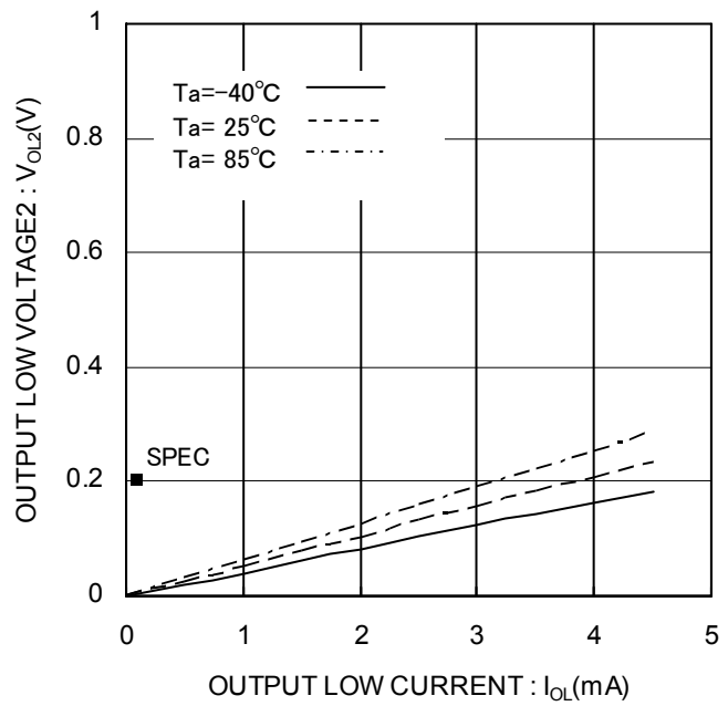
Figure 7. Output low voltage2 V_{O2} ( V_{CC}=1.7\text{V} )
