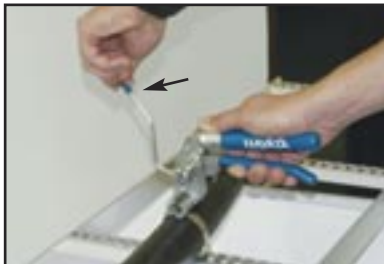
Push forward the Cutter Handle to trim the band.
