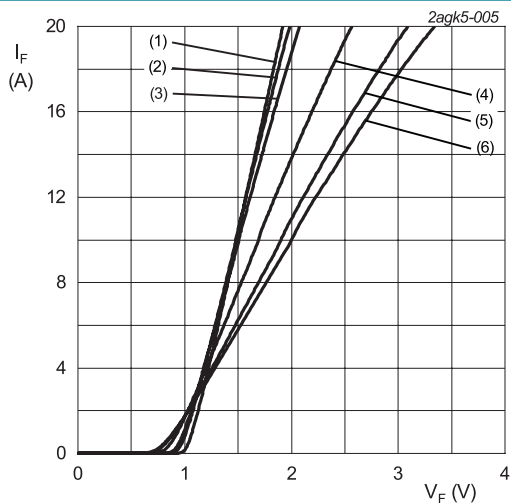
V_o = 1.916 \text{ V}; R_s = 0.0523 \text{ } \Omega (1) T_j = -55 \text{ }^\circ\text{C}; typical values (2) T_j = 0 \text{ }^\circ\text{C}; typical values (3) T_j = 25 \text{ }^\circ\text{C}; typical values (4) T_j = 100 \text{ }^\circ\text{C}; typical values (5) T_j = 150 \text{ }^\circ\text{C}; typical values (6) T_j = 175 \text{ }^\circ\text{C}; typical values
