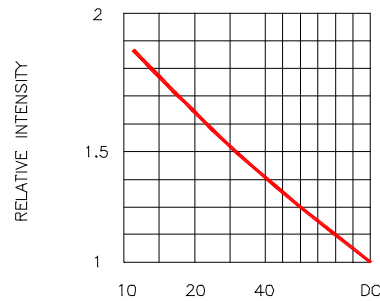
Fig.4 LUMINOUS INTENSITY VS. DUTY CYCLE (AVERAGE If=10mA)
