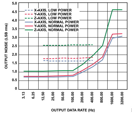
Figure 41. Noise vs. Output Data Rate for Normal and Low Power Modes, Full-Resolution (256 LSB/g)
