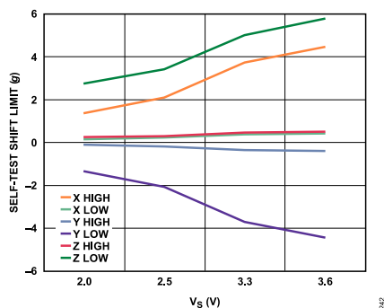
Figure 33. Self-Test Output Change Limits vs. Supply Voltage
