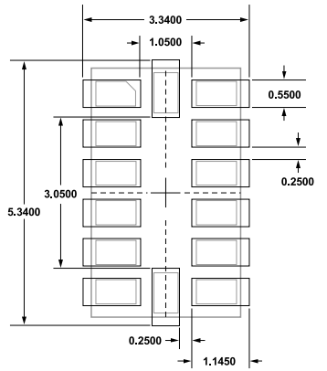
Figure 49. Recommended Printed Wiring Board Land Pattern (Dimensions shown in millimeters)
