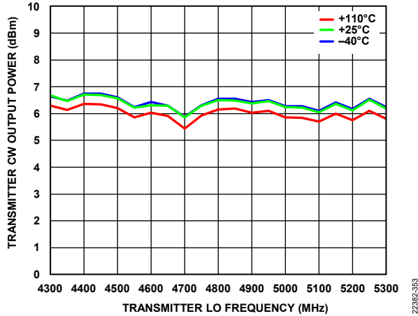
Figure 424. Transmitter CW Output Power vs. Transmitter LO Frequency, 10 MHz Offset, 0 dB Attenuation
