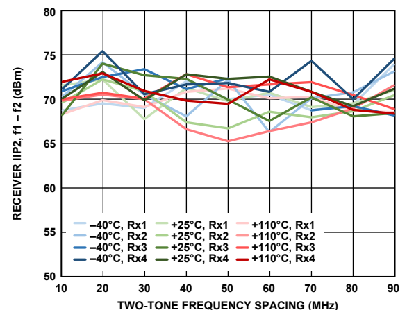
Figure 204. Receiver IIP2, f_1 - f_2 vs. Two-Tone Frequency Spacing, Both Tones at -11 dBFS, f_2 = 2 MHz
