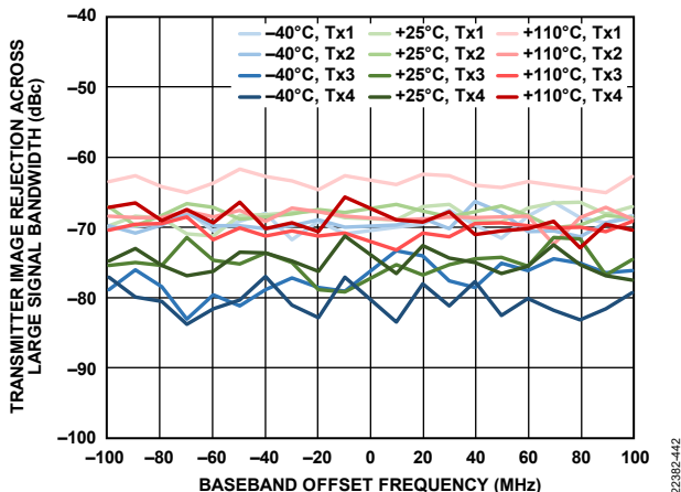
Figure 513. Transmitter Image Rejection Across Large Signal Bandwidth vs. Baseband Offset Frequency
