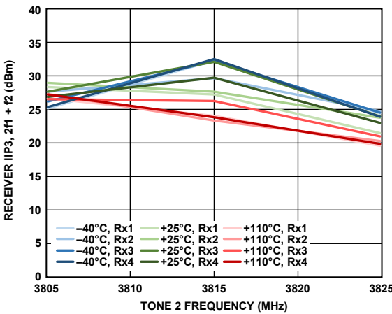
Figure 381. Receiver IIP3, 2f_1 + f_2 vs. Tone 2 Frequency, Both Tones at -11 dBFS, f_1 = f_2 + 2 MHz
