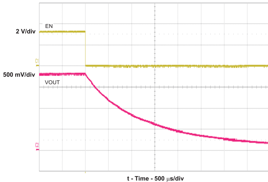
Figure 8. TPS62060 Shutdown With No Load
