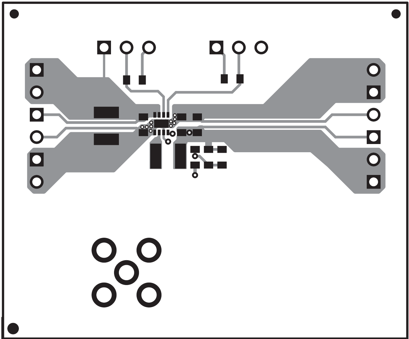
Figure 18. TPS62060EVM Top-Side Copper, Top View
