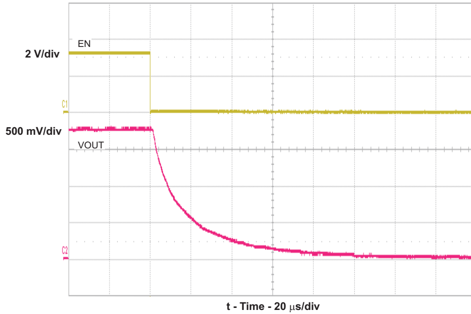
Figure 7. TPS62060 Shutdown Into 2.2- \Omega Load
