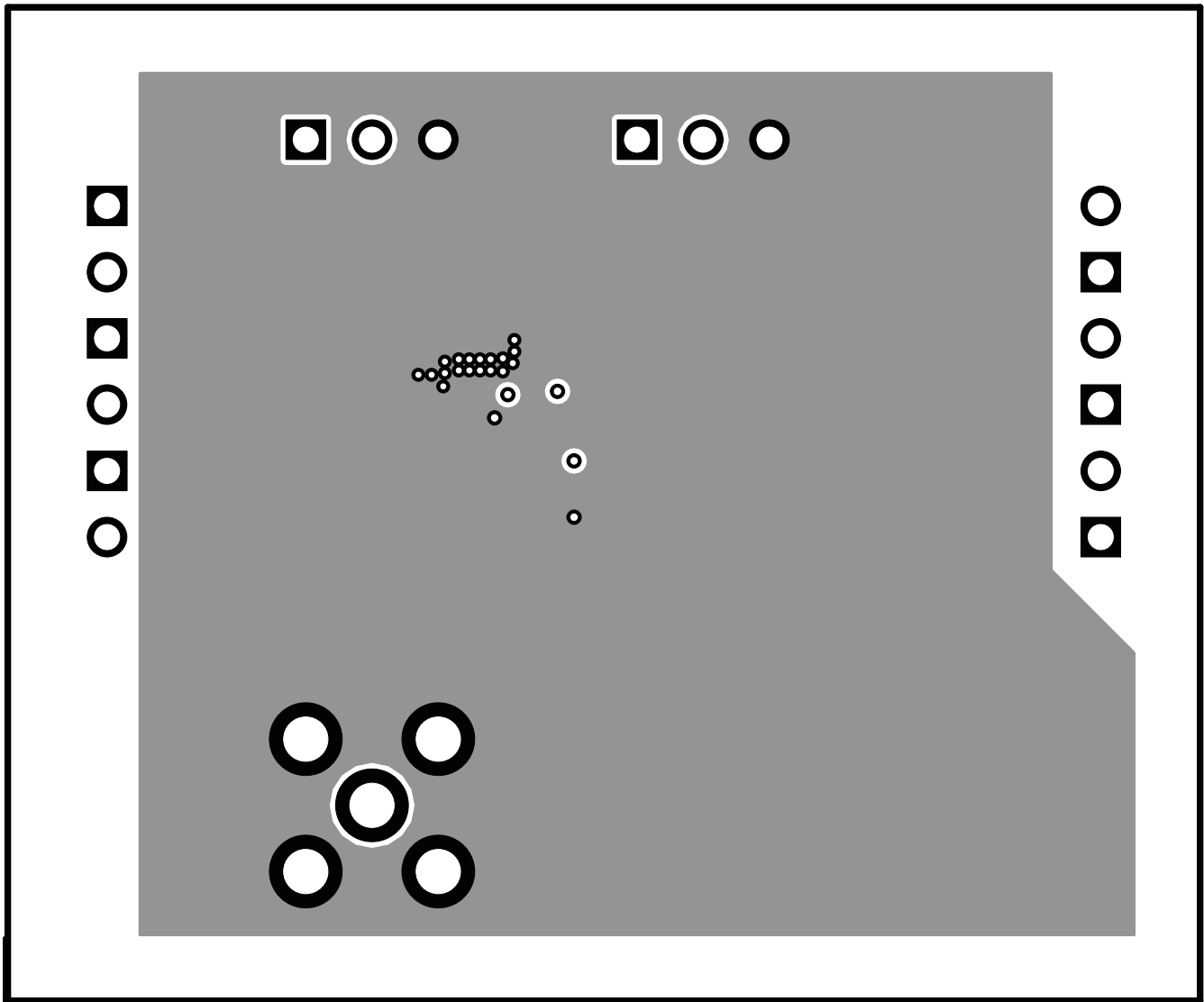
Figure 19. TPS62060EVM Internal Layer 1, X-Ray View From Top
