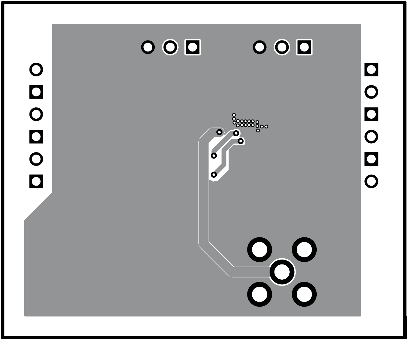
Figure 21. TPS62060EVM Bottom-Side Copper, Bottom View
