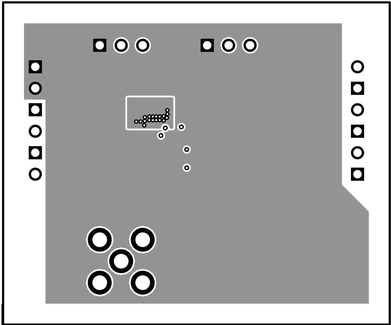
Figure 20. TPS62060EVM Internal Layer 2, X-Ray View From Top
