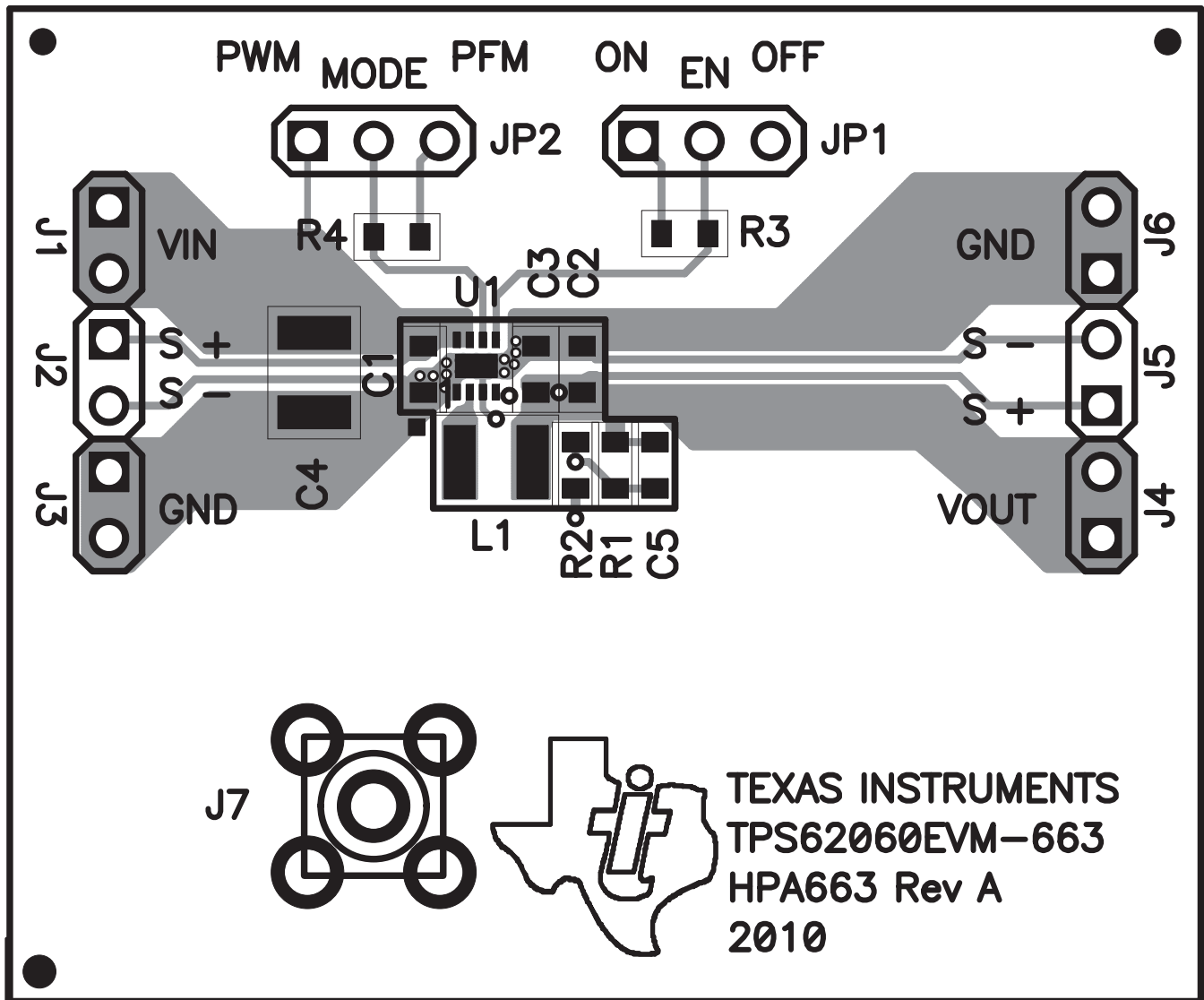
Figure 17. TPS62060EVM Component Placement, Top View
