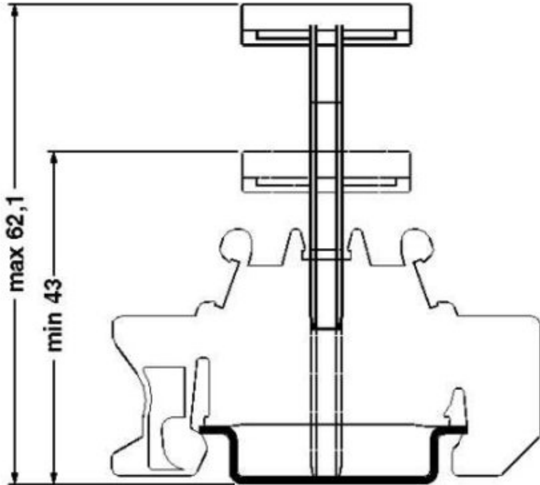
Dimensional drawing
