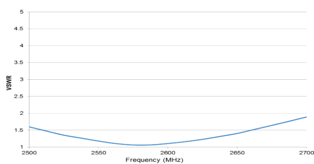
High High Band VSWR
