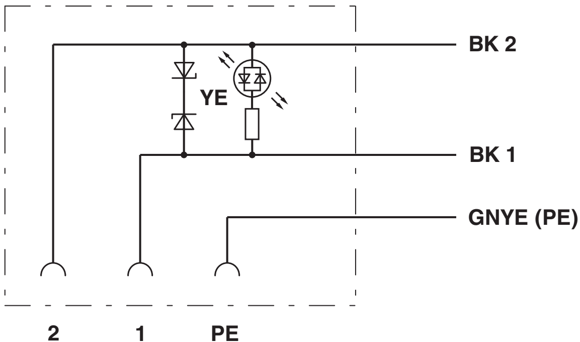
Circuit diagram
