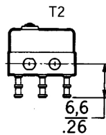
STRAIGHT PIN
