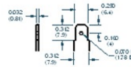
"Q" TERMINALS
