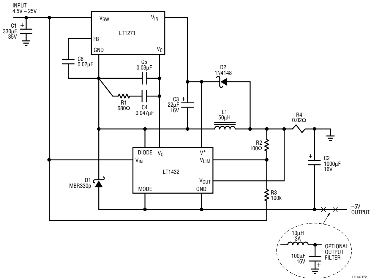
Figure 22. Positive-to-Negative Converter
