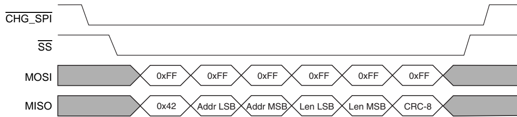
FIGURE 9-8: SPI_READ_FAIL
