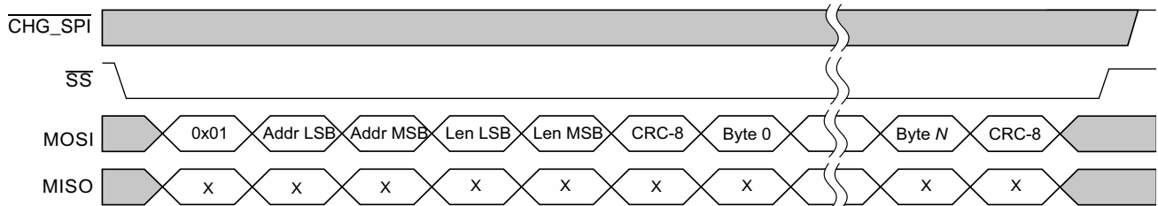
FIGURE 9-2: SPI_WRITE_REQ
