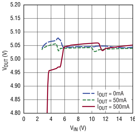
5V Fixed Output Voltage vs Input Voltage
