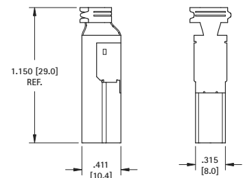
CABLE PLUG
