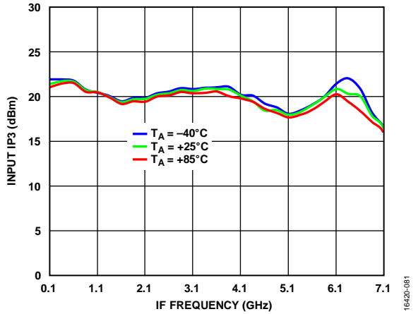
Figure 79. Input IP3 vs. IF Frequency at Various Temperatures, LO = 13 dBm
