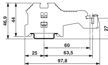
Dimensioned drawing
