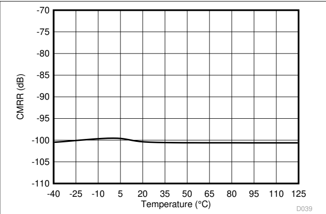
Figure 6-12. Common-Mode Rejection Ratio vs Temperature
