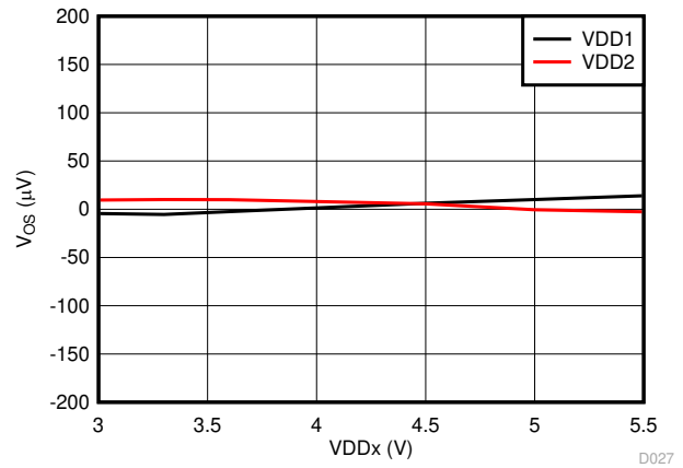
Figure 6-8. Input Offset Voltage vs Supply Voltage
