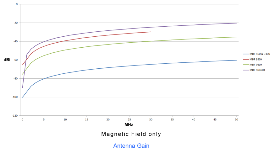
Antenna Gain
