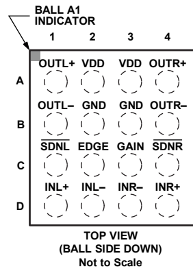
Figure 2. Pin Configuration (Top Side View)
