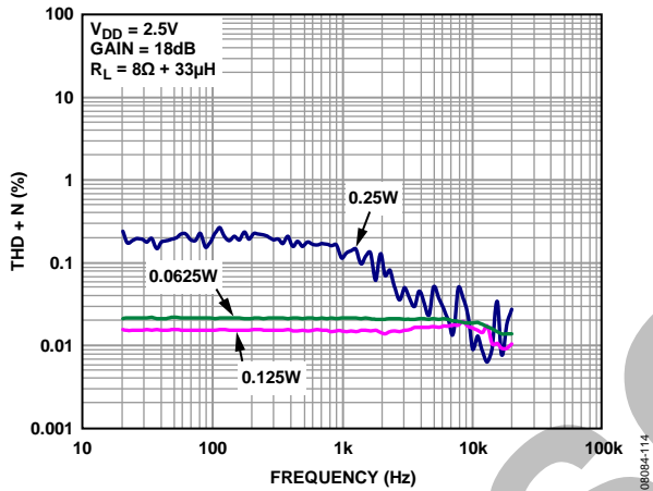
Figure 16. THD + N vs. Frequency, V_{DD} = 2.5V , R_L = 8\Omega , A_v = 18dB
