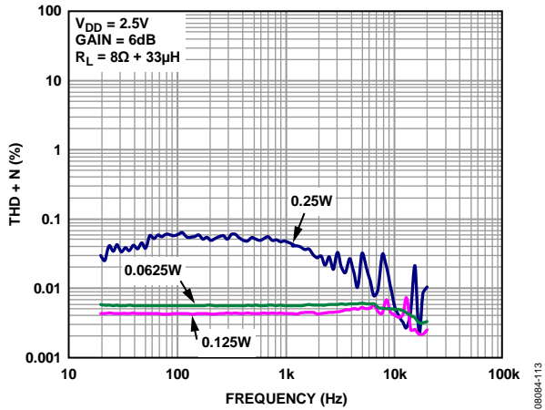
Figure 15. THD + N vs. Frequency, V_{DD} = 2.5V , R_L = 8\Omega , A_v = 6dB
