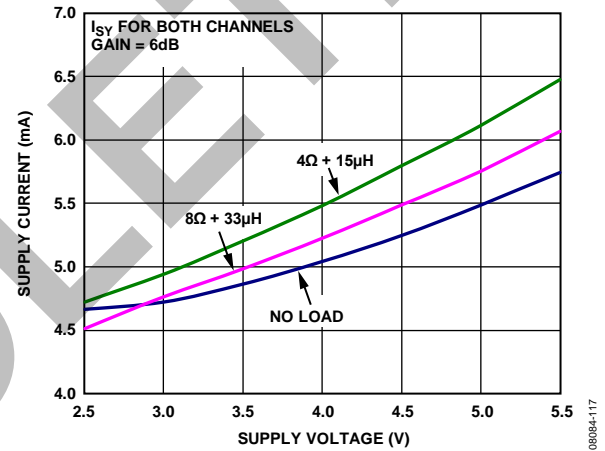
Figure 19. Supply Current vs. Supply Voltage, A_v = 6dB
