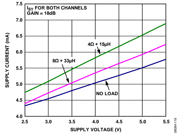
Figure 20. Supply Current vs. Supply Voltage, A_v = 18dB
