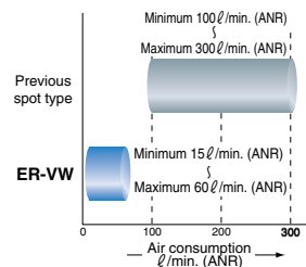
Comparison of air consumption
